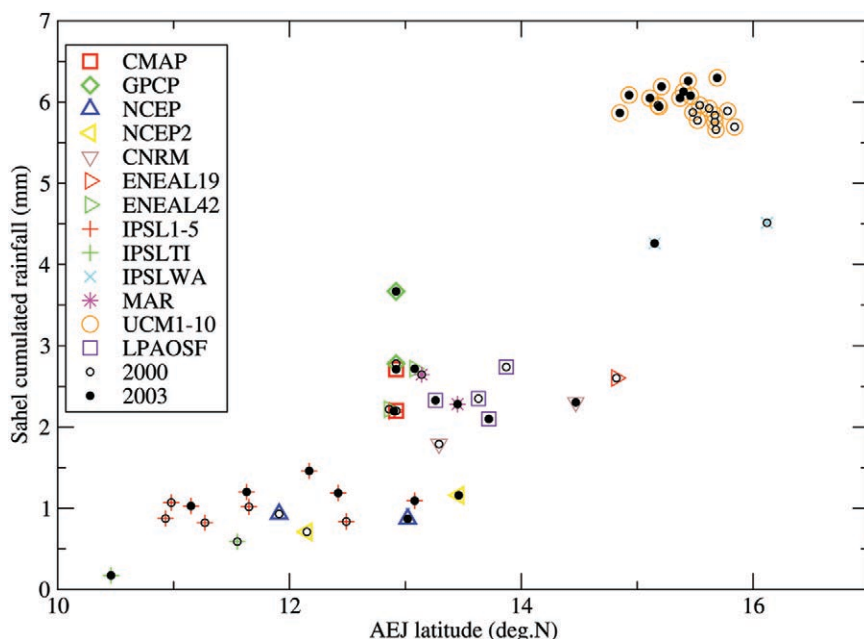
FIG. 5. Latitude of AEJ ( ^{\circ}\text{N} ) versus mean rainfall over a Sahelian box ( 13^{\circ}\text{--}18^{\circ}\text{N} , 10^{\circ}\text{W}\text{--}10^{\circ}\text{E} ) for all of the AMMA-MIP simulations; for the CMAP and GPCP observations; and NCEP–NCAR, and NCEP-2 reanalyses for JJAS season, and 2000 (empty circle) and 2003 (filled circle) years. The AEJ latitude for CMAP and GPCP corresponds to the ERA-40 reanalyses for year 2000 and to ERA-Interim reanalyses for year 2003.
